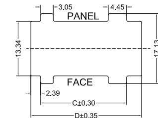
PANEL OPENING RECOMMENDED PANEL THICKNESS 1.57/1.27
