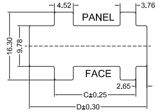
PANEL OPENING RECOMMENDED PANEL THICKNESS 1.57/1.27
