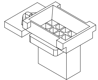
PANEL OPENING RECOMMENDED PANEL THICKNESS 1.57/1.27
