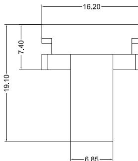
PANEL OPENING RECOMMENDED PANEL THICKNESS 1.57/1.27
