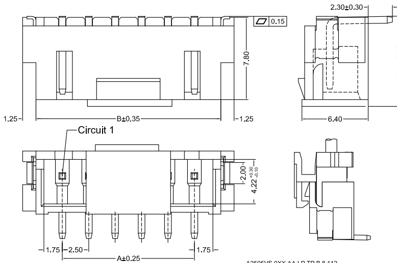
Recommended P.C.B Layout General Tolerance±0.05
