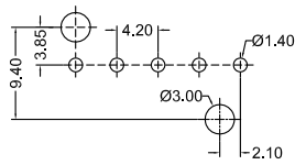
Recommended P.C.B Layout General Tolerance±0.05
