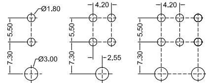
Recommended P.C.B Layout General Tolerance±0.05
