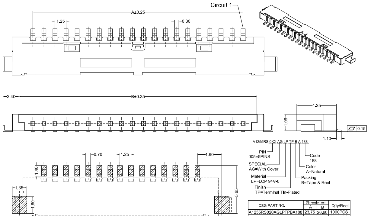
Recommended P.C.B Layout General Tolerance±0.05
